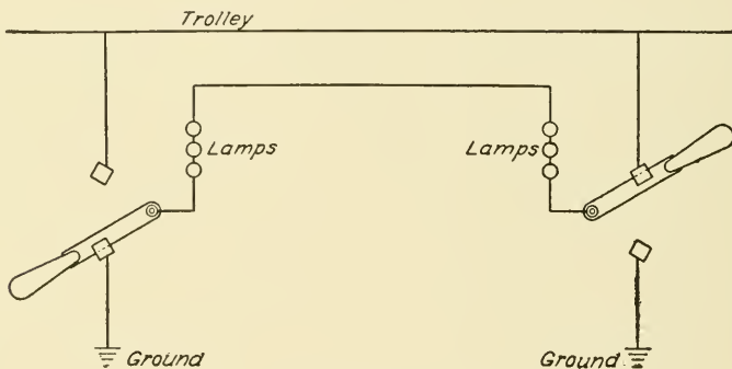
Fig. 212. Hand-Operated Block System
